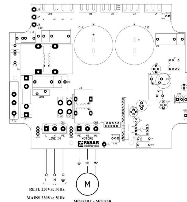
Connection scheme
